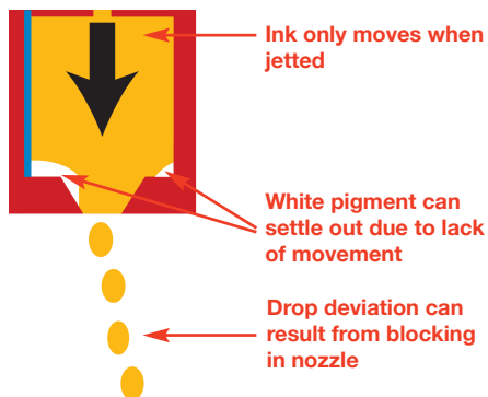
Figure 4: Ink sedimentation in end-shooter printhead
