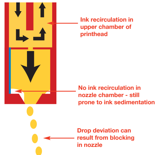
Figure 5: Ink sedimentation in end-shooter printhead with internal ink recirculation
