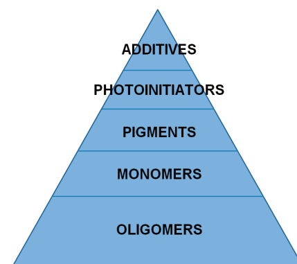
Figure 3: Typical formulation of a UV curable ink
