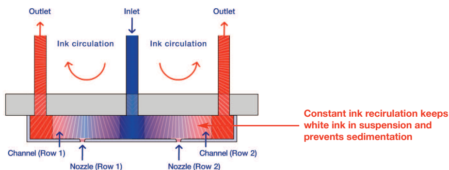
Figure 6: Constant ink recirculation prevents ink sedimentation and consequential nozzle blocking
